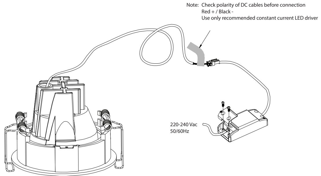
CONNECTION DRAWING
