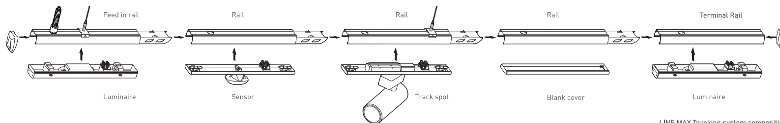
LINE MAX Trunking system composition
